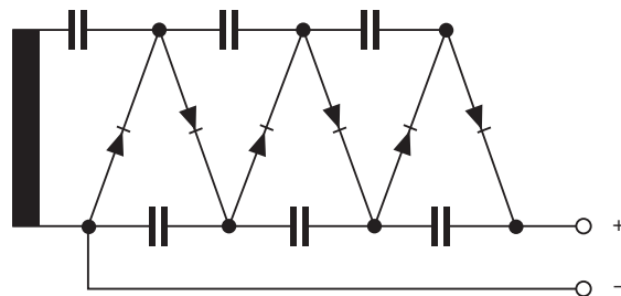
Half-wave-multiplier
